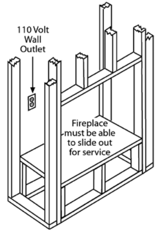
(B) Raised Framing
