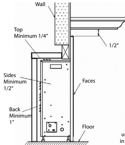
Clearances To Combustibles
